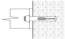
Shown with M8 x 40mm Shear Nuts
